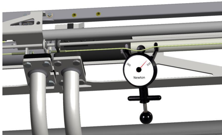
Figure 26: Tension meter
