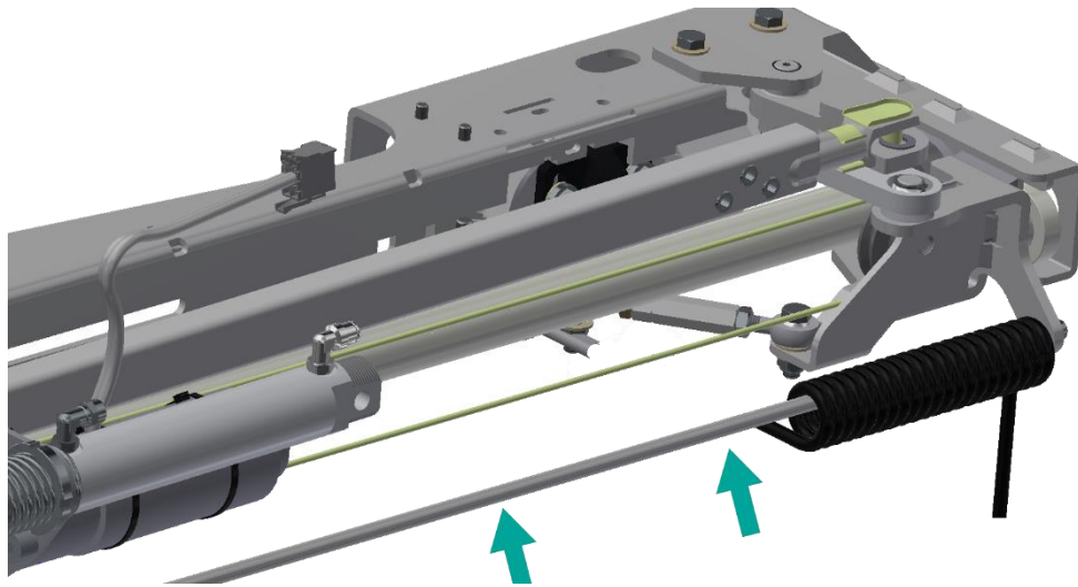
Figure 28: Spiral cable guiding shaft
