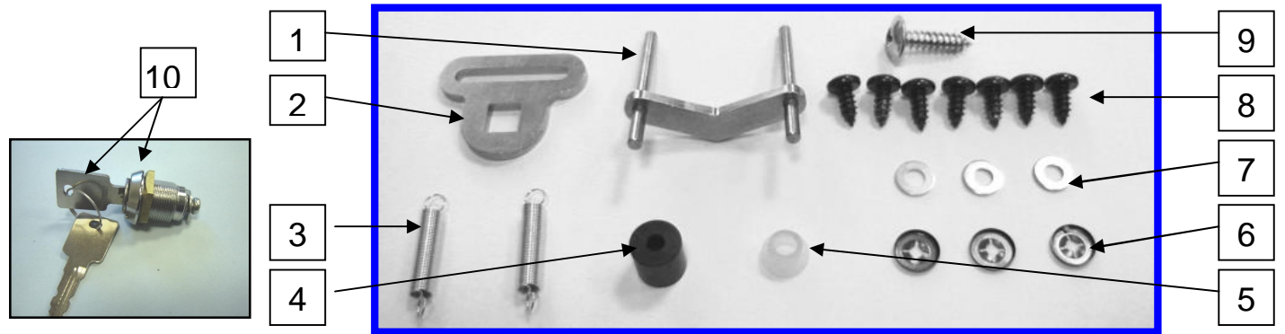
LCK112-KIT= Lock Kit comprising of items 1 to 10
