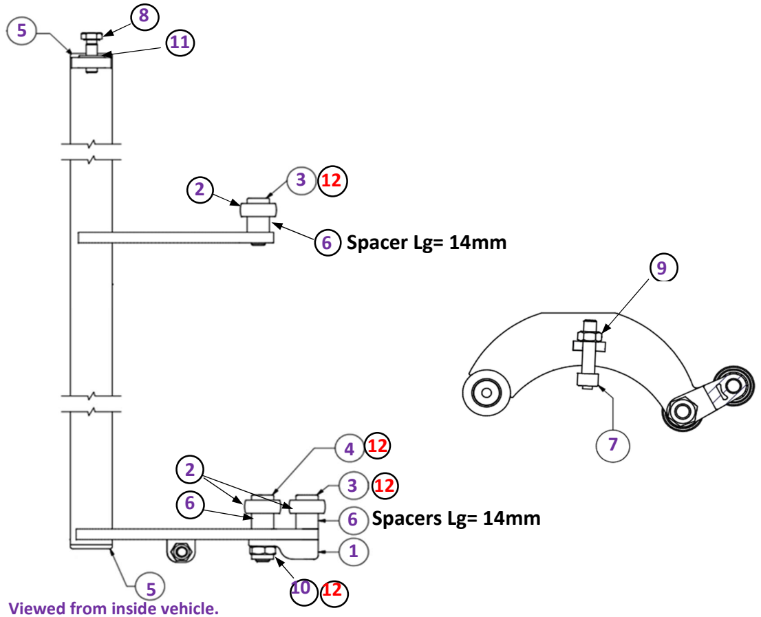
TYPICAL LH DOORSHAFT AS SHOWN, RH OPPOSITE HAND
