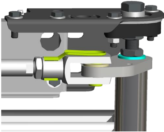
Figure 2: Secure nut with SK ring
