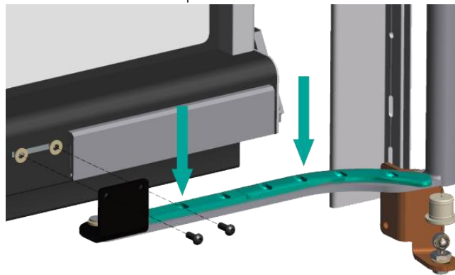
Figure 8: Sliding plate
