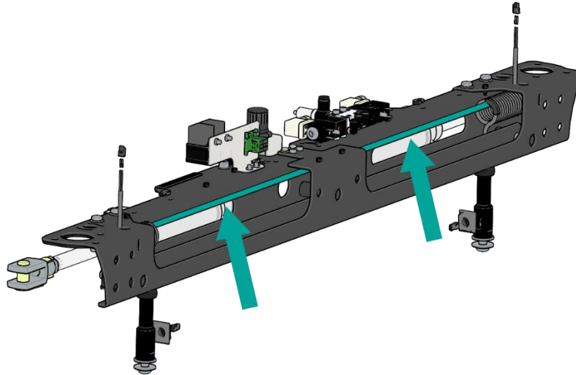
Figure 11: Spiral cable guiding shaft
