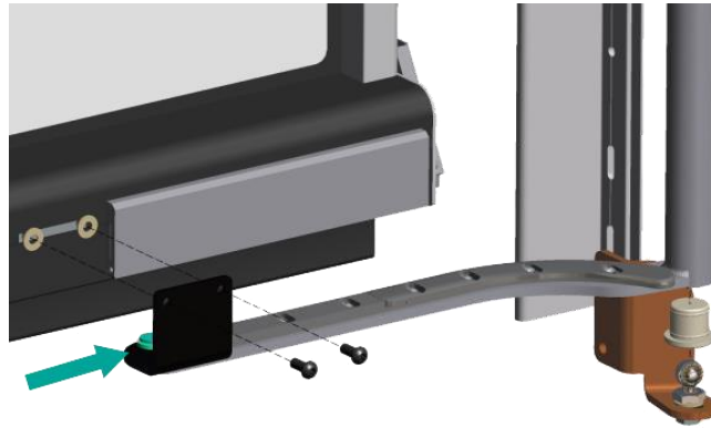
Figure 7: Lever bearing bush
