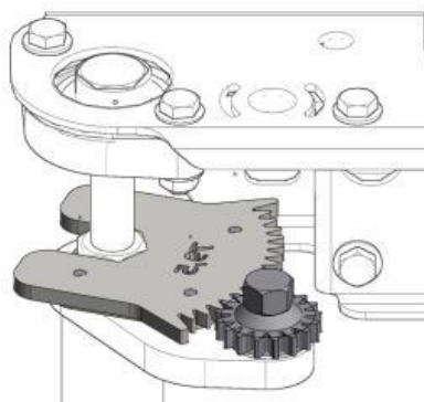
Figure 4: VA3860 Torque Wrench
