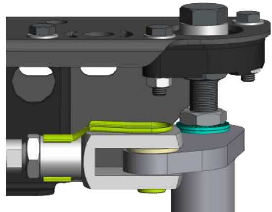
Figure 3: Secure nut with Nord-lock
